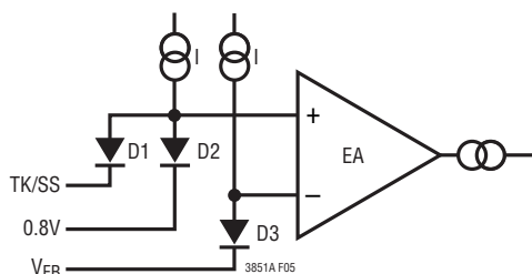
Figure 5. Equivalent Input Circuit of Error Amplifier
